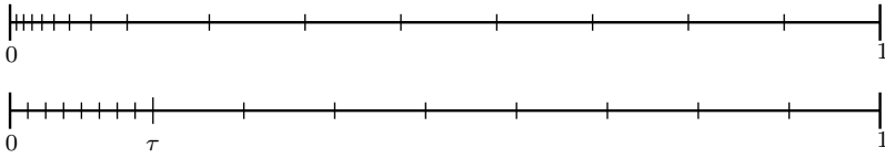
Fig. 2.4 Bakhvalov mesh (top) and Shishkin mesh (below) for a convection-diffusion equation
