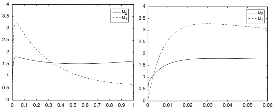
Fig. 3.2 Overlapping layers in a system of two reaction-diffusion equations
